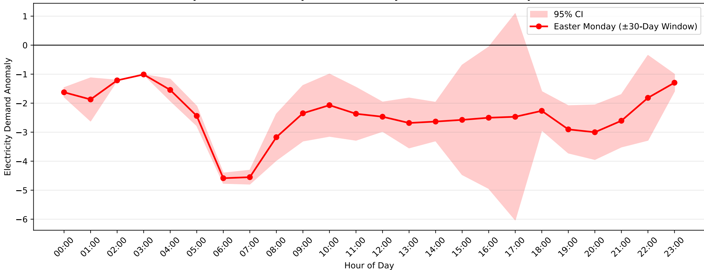
Revesby Demand Anomaly: Easter Monday (2009–2010, \pm 30 -Day Window)
