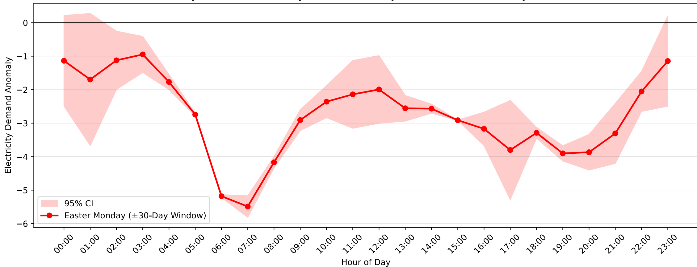
Revesby Demand Anomaly: Easter Monday (2010-2011, \pm 30 -Day Window)
