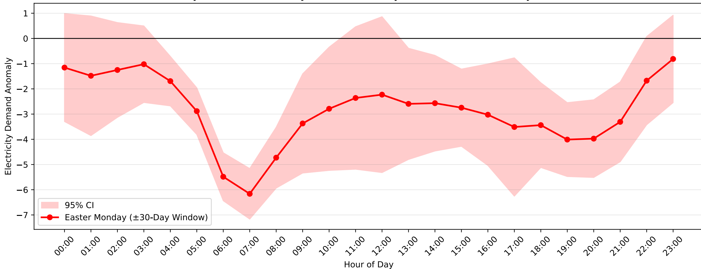
Revesby Demand Anomaly: Easter Monday (2011-2012, \pm 30 -Day Window)
